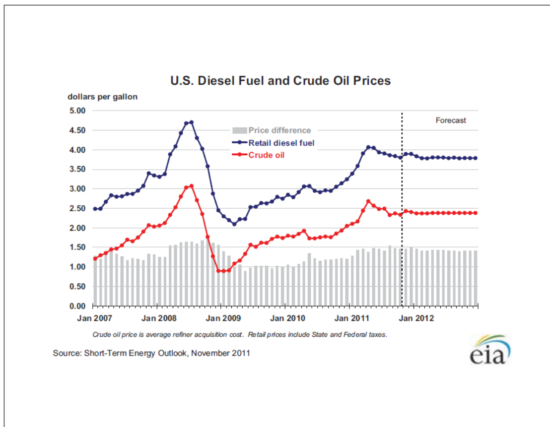
Figure 15. Price ranges for crude oil (yearly average).
