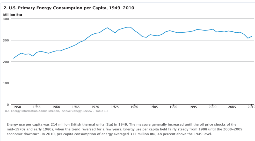
Figure 2. Overall energy consumption and consumption per capita in the United States over last half century. 30
