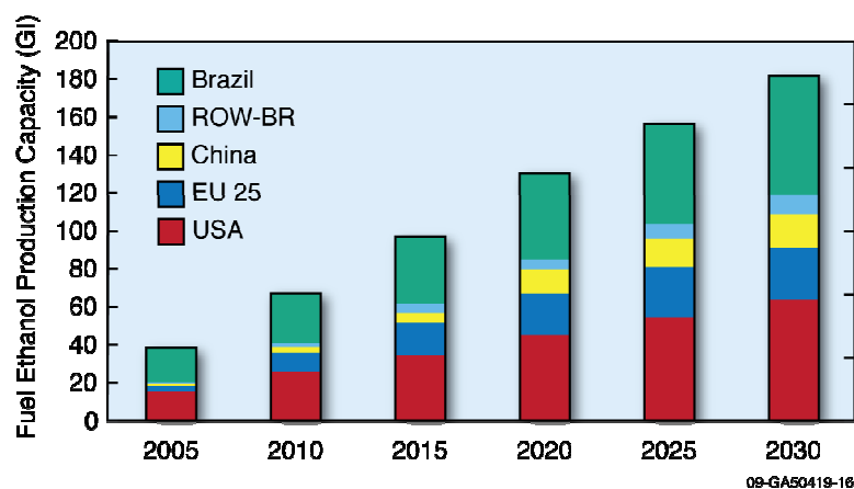
Figure 24. Estimated fuel ethanol capacity of production (conventional technologies). 109
