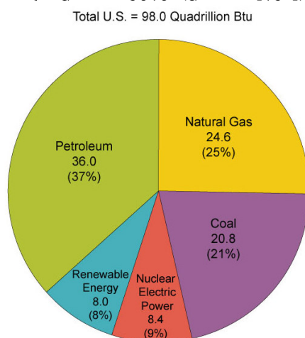
Figure 20. Primary energy use by Source, 2010. (Source: [12a]) (Quadrillion Btu and Percent)
