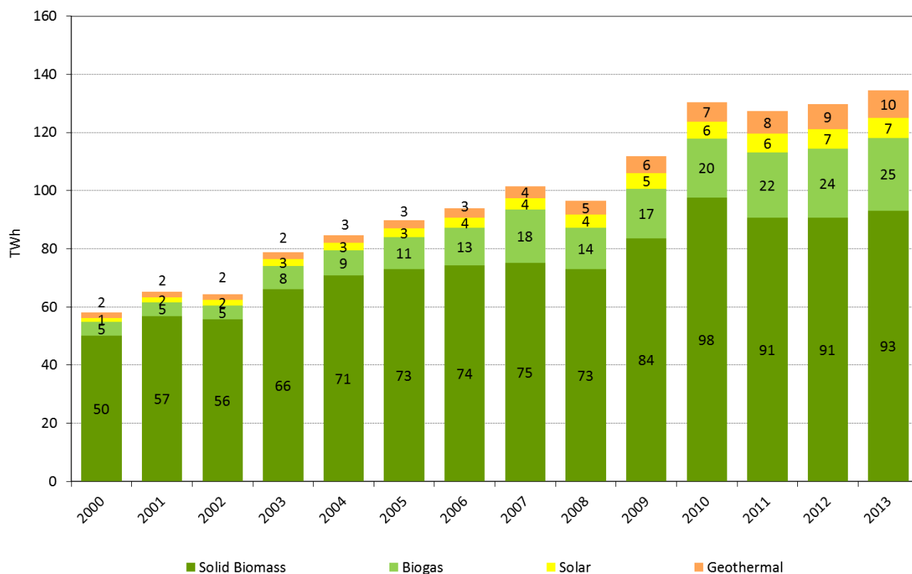
Figure 1-10: Renewable Heat Supply by Source in Germany 2000-2013 (BMWi 2014)
