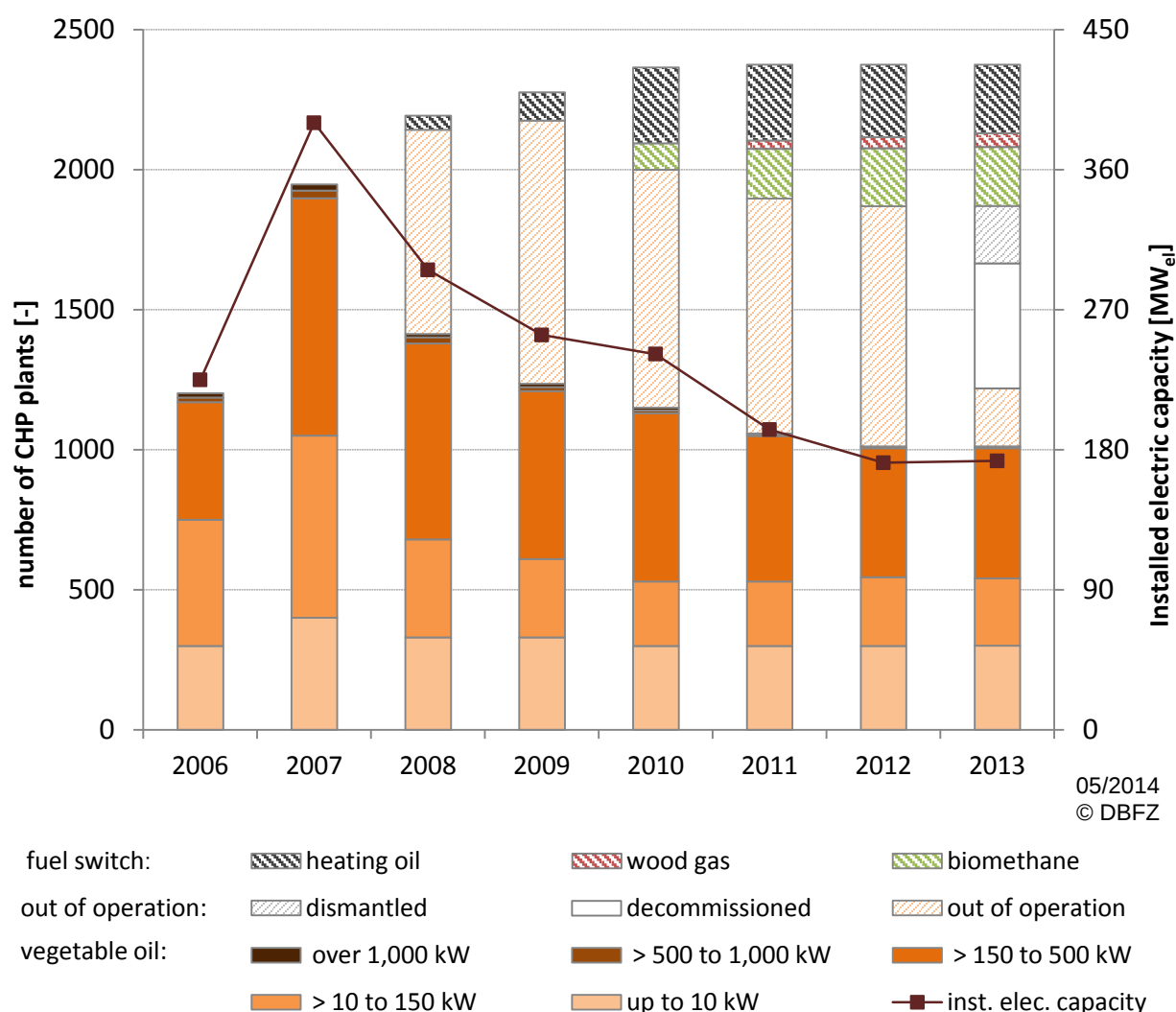
Figure 2-17: Development of vegetable oil CHP plants in Germany from 2006 to 2013 (number of plants and installed electric capacity in MW el ) (DBFZ, 2014)
