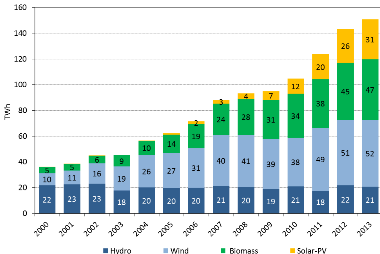
Figure 1-9: Renewable Electricity Generation by Source in Germany 2000-2013 (BMWi 2014)
