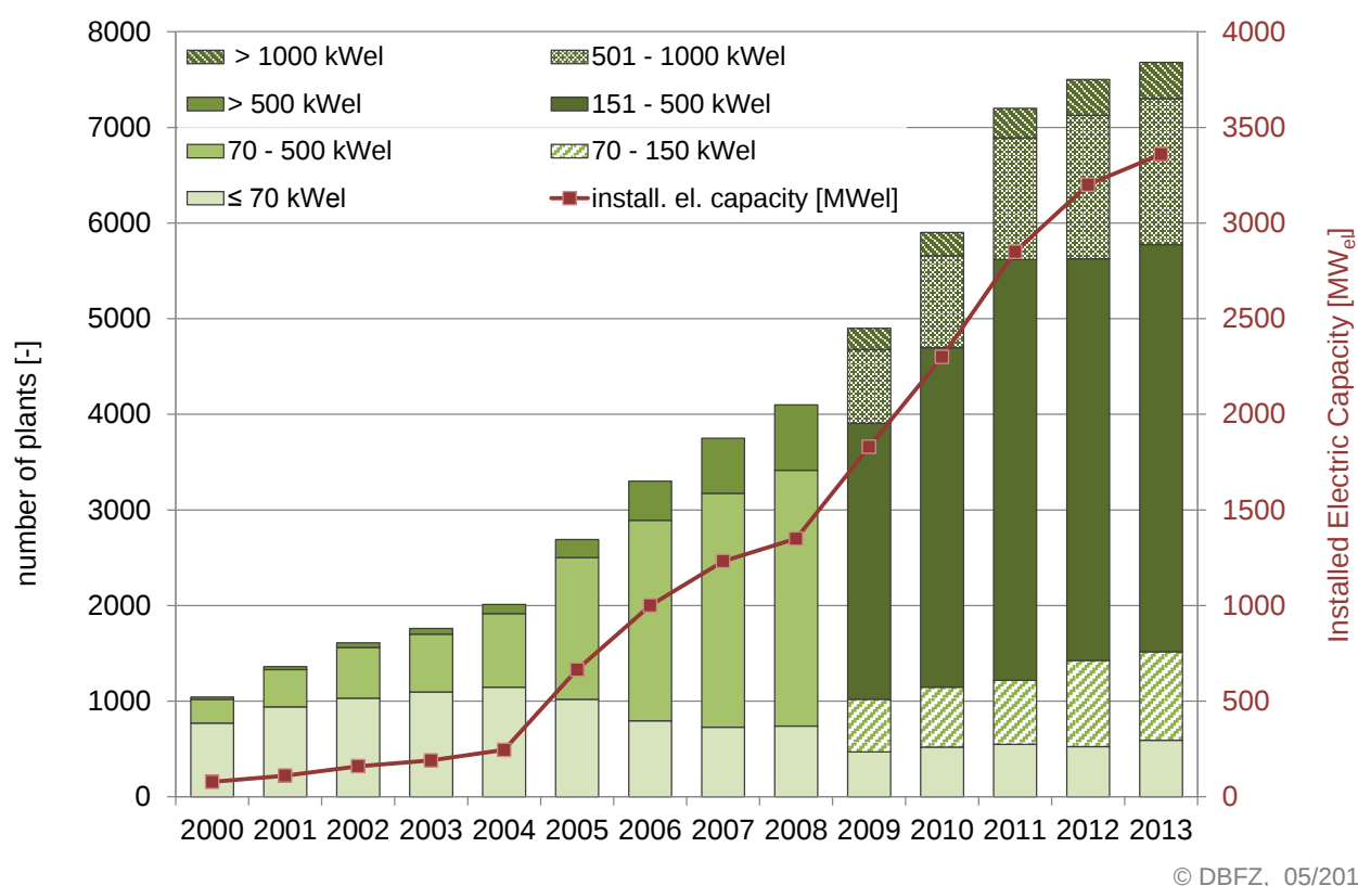
Figure 2-1: Development of biogas plants in Germany (number of plants and installed electric capacity in MW el ) from 2000 to 2013, without biogas upgrading plants, landfill and sewage gas plants (DBFZ, 2014)
