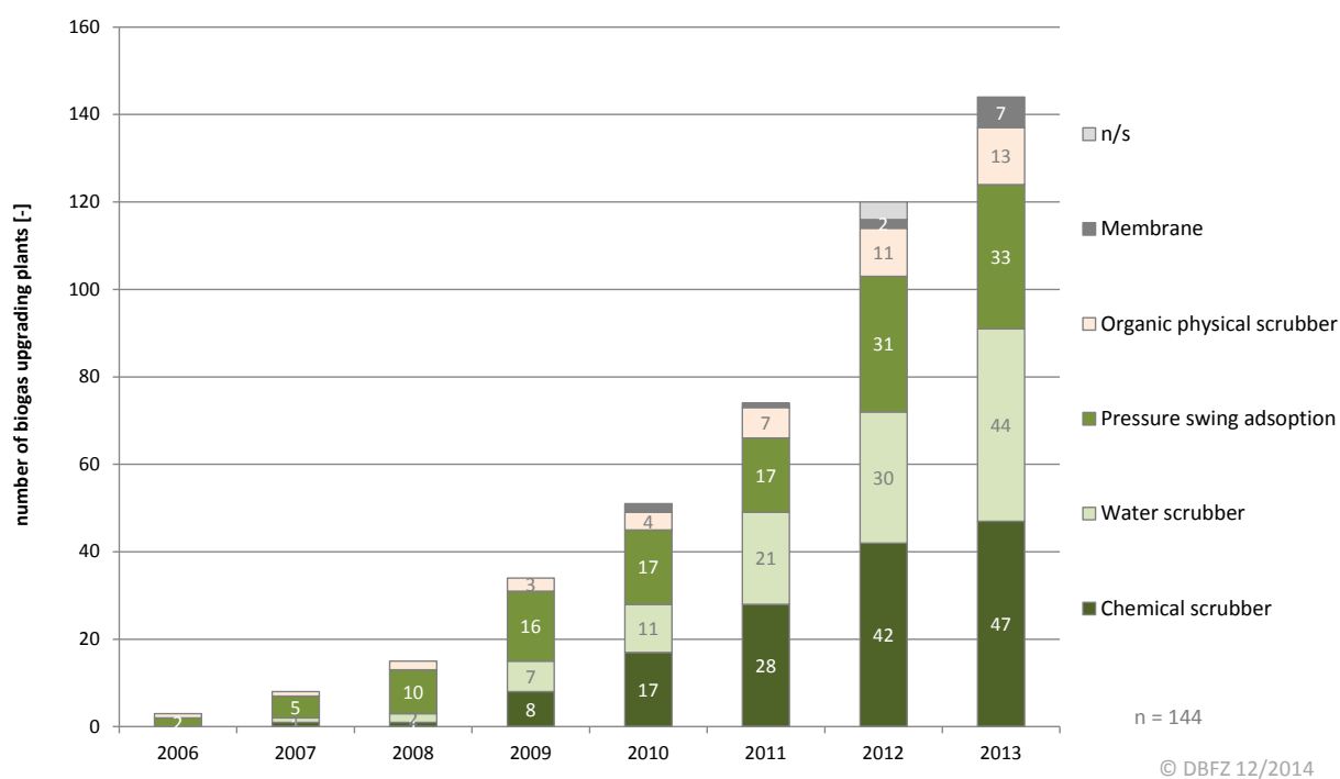
Figure 2-9: Biogas upgrading technologies in Germany from 2006 to 2013 (DBFZ, 2014)
