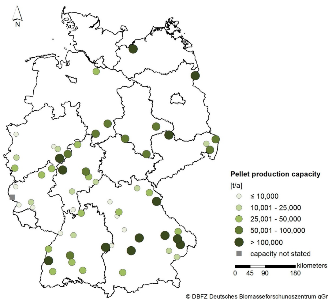
Figure 2-16: Distribution of wood pellet production plants in Germany in 2013 (this overview makes no claim of being complete) (Solar Promotion GmbH, 2013) (C.A.R.M.E.N. e.V., 2014a)
