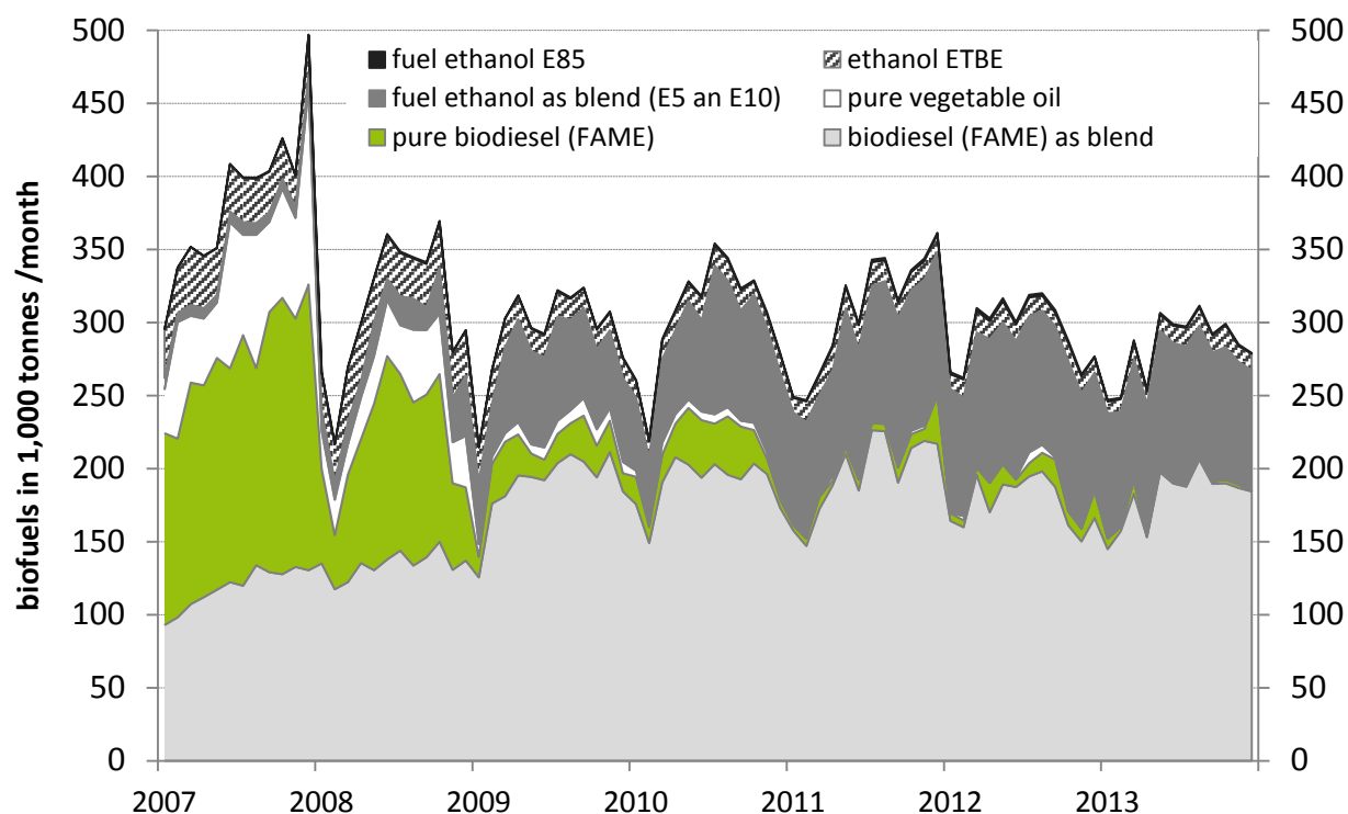
Figure 2-18: Development of the biofuel consumption in Germany from 2007 to 2013 (Naumann et al., 2014)
