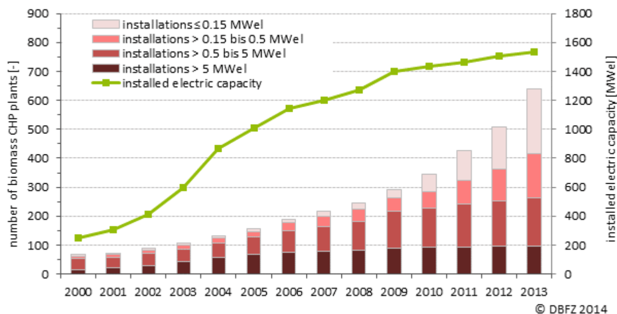
Figure 2-11: Development of solid biomass CHP plants in Germany from 2000 to 2013 (number of plants and installed electric capacity in MW el ), without installations of the pulp and paper industry and small-scale CHP plants (< 10 kW el ) (DBFZ, 2014)
