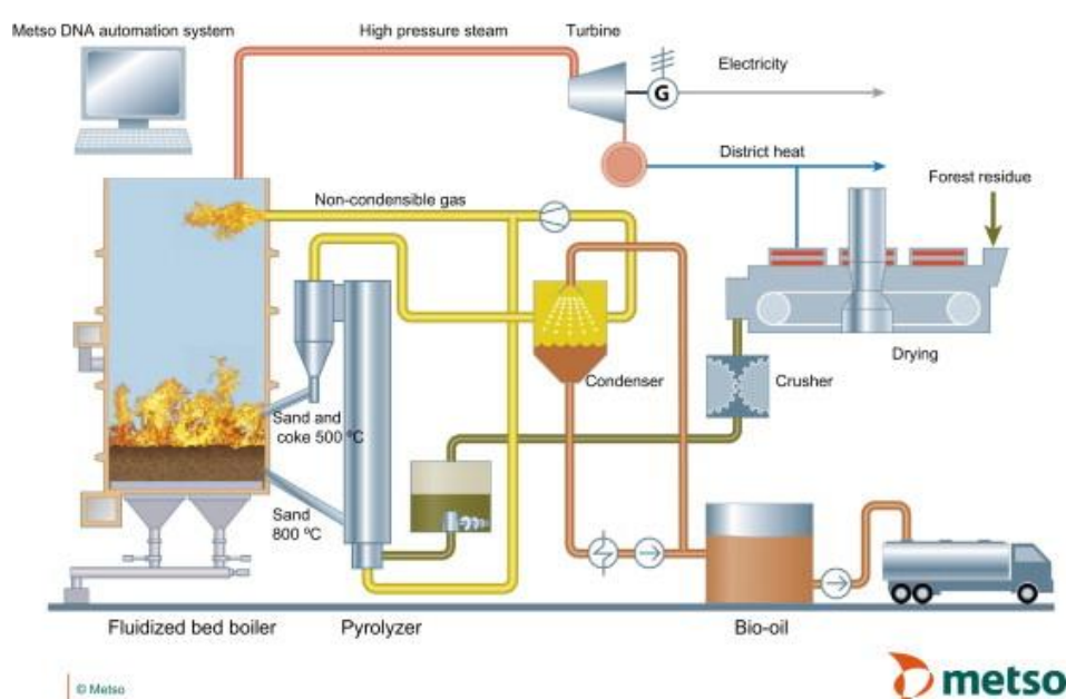
Figure 6-1 Fortum's fast pyrolysis plant for bio-oil production to be built in Joensuu, Finland.
