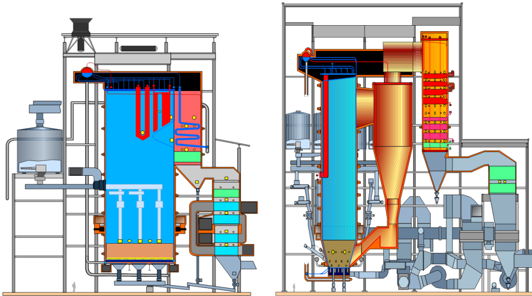
Figure 5-6 Fluidized bed boilers; bubbling fluidized bed (BFB) on the left and Circulating fluidized bed (CFB) on the right.
