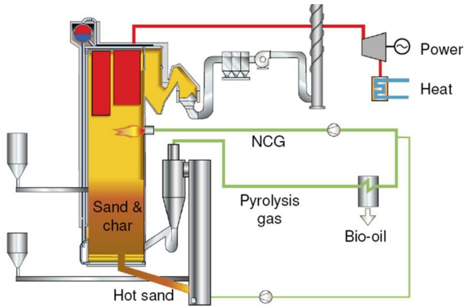
Figure 5-3. Integrated pyrolyser by VTT, Metso, UPM and Fortum [65].
