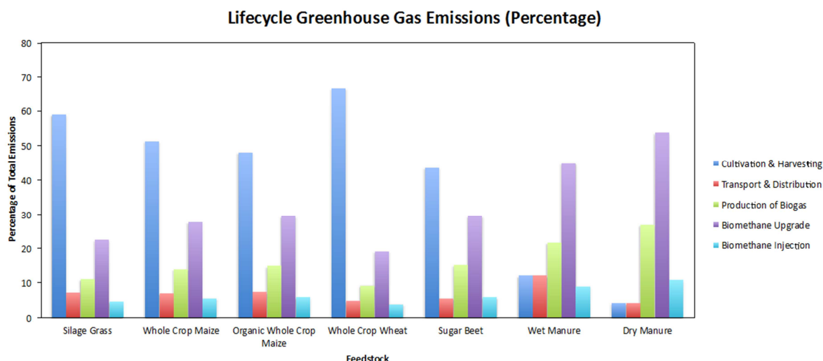
Figure 3-4. Percentage Lifecycle Emissions by Feedstock, calculated by using the UK Biomass Carbon Calculator Model (GGG, 2013a)
