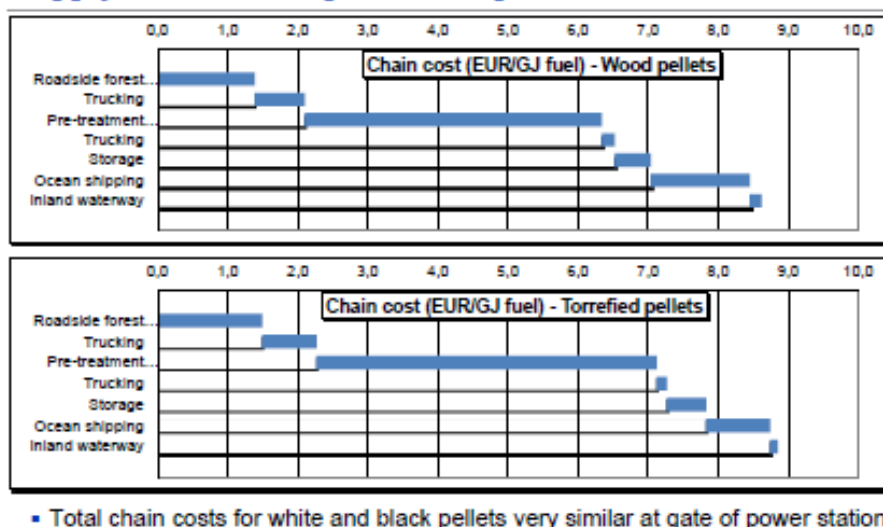
Figure 5 total chain costs white pellets versus black pellets
